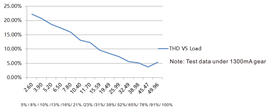
THD VS Load
