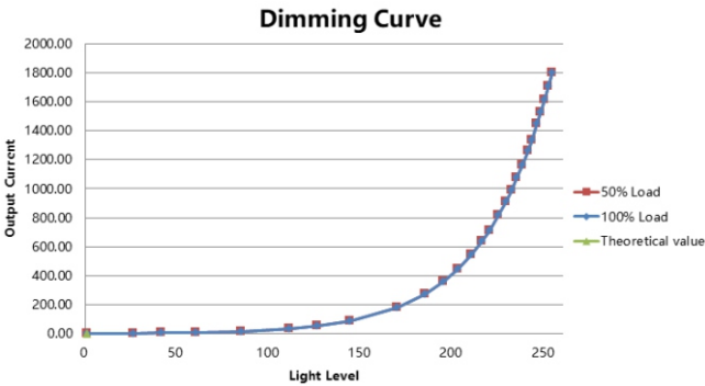
Dimming Curve
