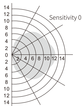
Wall Pattern (Unit: m) Installation Height: 2.5m
