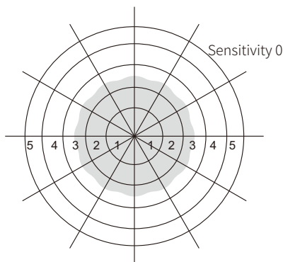
Ceiling Pattern (Unit: m) Installation Height: 2.5m
