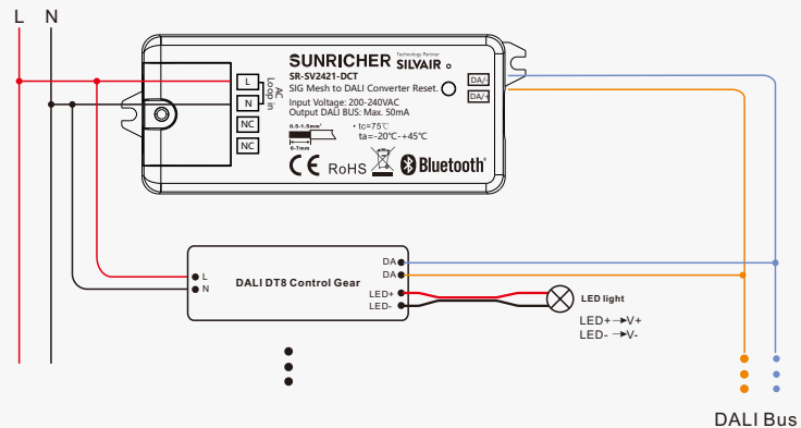
2) SR-SV2421-DCT Diagram (With DT8 Device)
