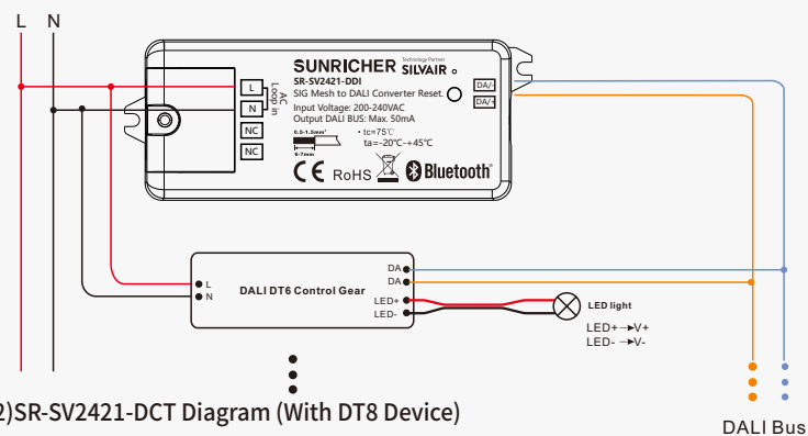
1) SR-SV2421-DDI Diagram (With DT6 Device)
