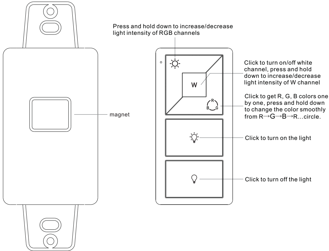
Bracket
