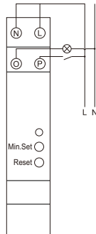
Method 2: Without neutral
