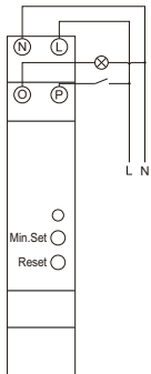
Method 1: With neutral
