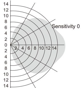
Wall Pattern (Unit: m) Installation Height: 10m
