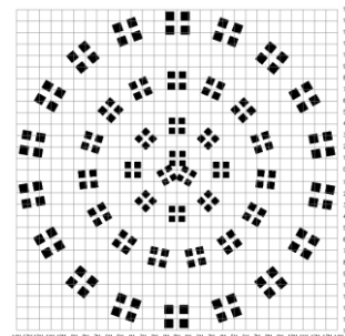
High-bay lens detection pattern at 12m
