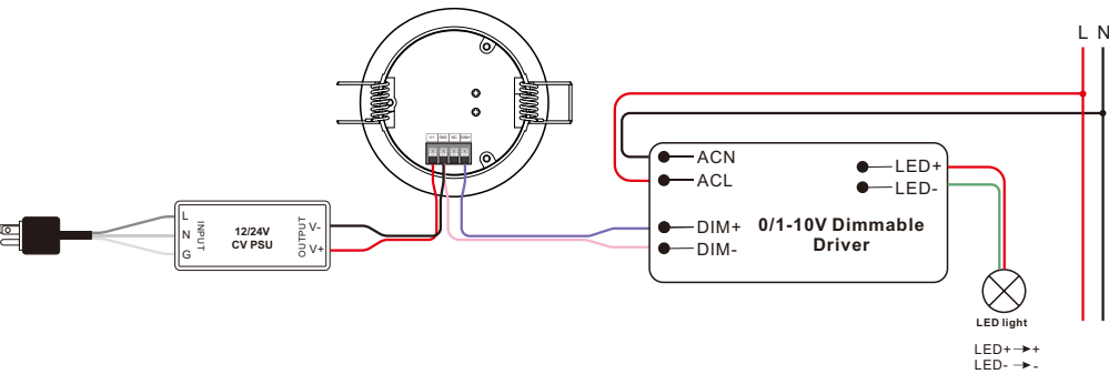
Wiring Diagram
