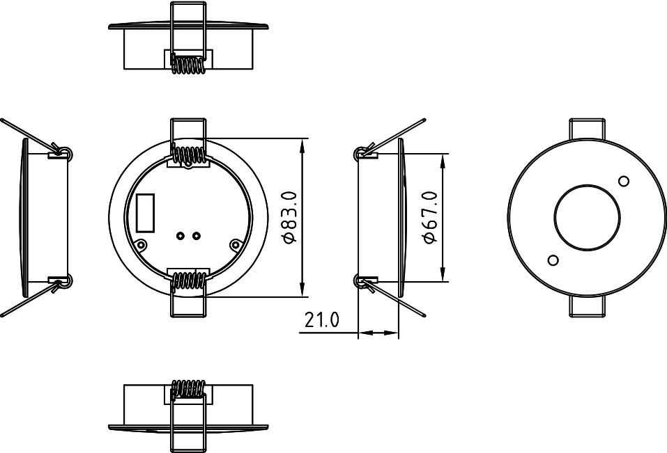
Product Dimension
