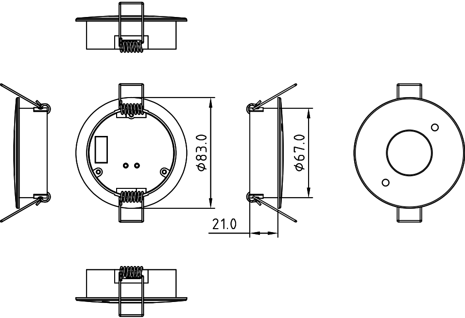
Product Dimension
