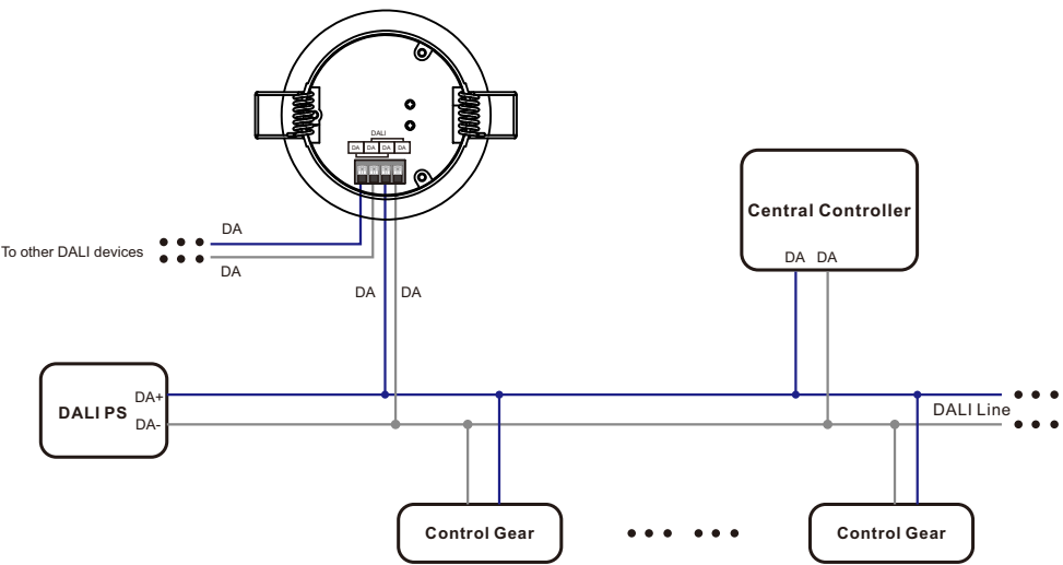
Wiring Diagram
