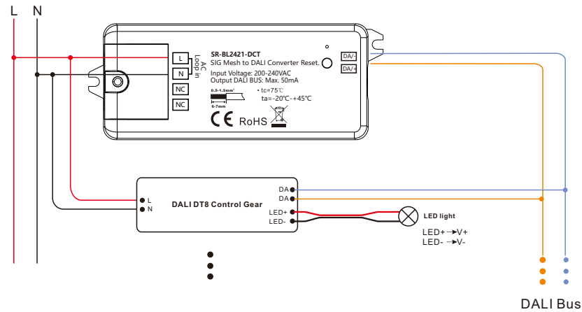
2)SR-BL2421-DCT Diagram (With DT8 Device)
