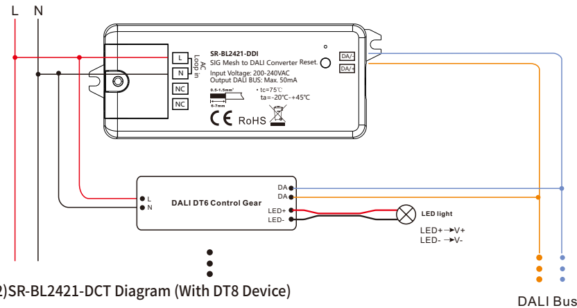
1)SR-BL2421-DDI Diagram (With DT6 Device)
