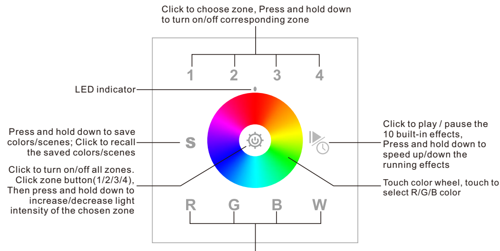
Front side
