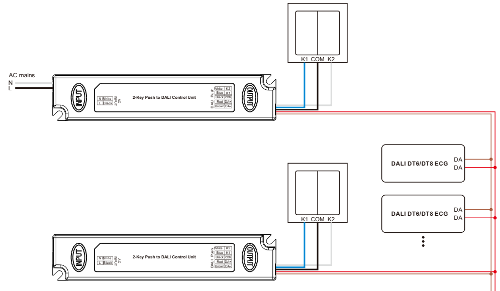
Figure 2: Wiring scheme to control up to 50 DALI ECGs (2 control units powered by AC mains, 3 control units powered by AC mains for 75 DALI ECGs, 4 control units powered by AC mains for 100 DALI ECGs)
